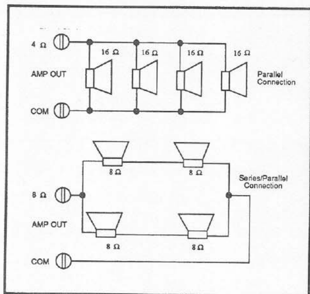
Figure 3 - Speaker Configurations
