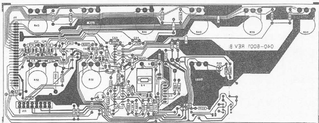
Mixer Preamp Board 9000 Series
